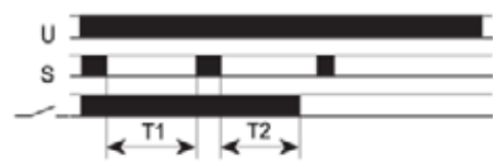
FZ11: Signal ON pulse + OFF pulse
